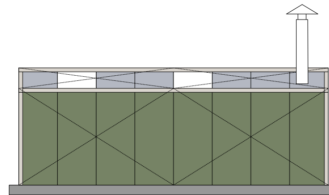
Right Elevation (Scale = 1:100)
