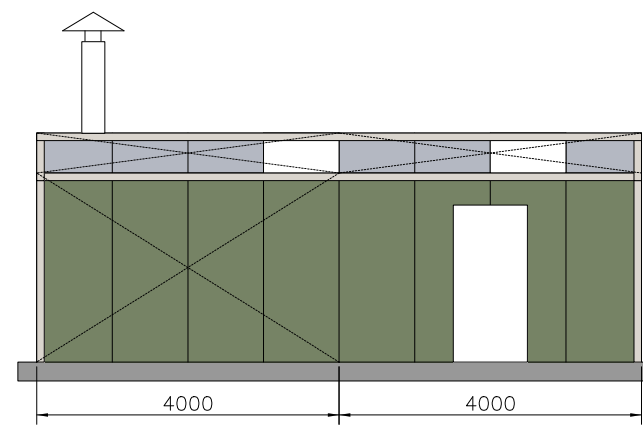
Left Elevation (Scale = 1:100)
