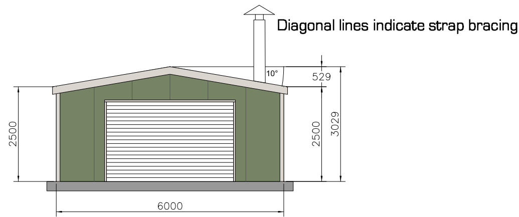
Front Elevation (External)
